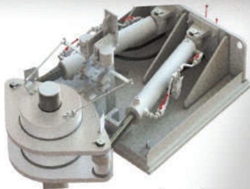
Steering Gear
